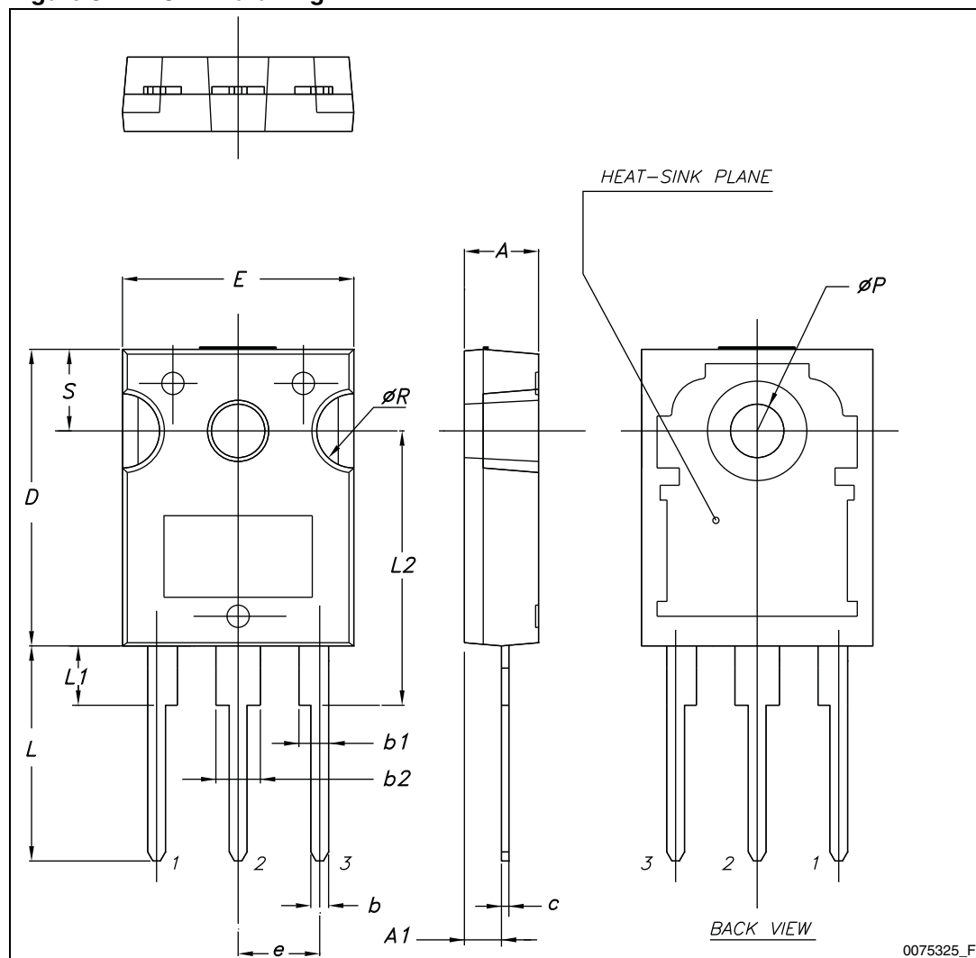
Figure 8. TO-247 drawing
